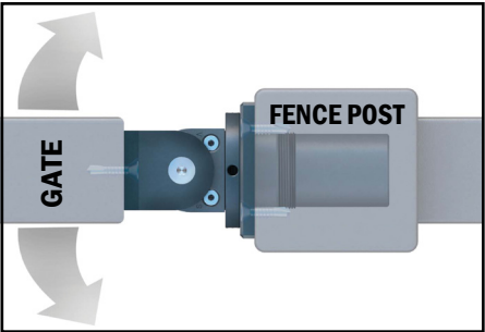
Center Mount
