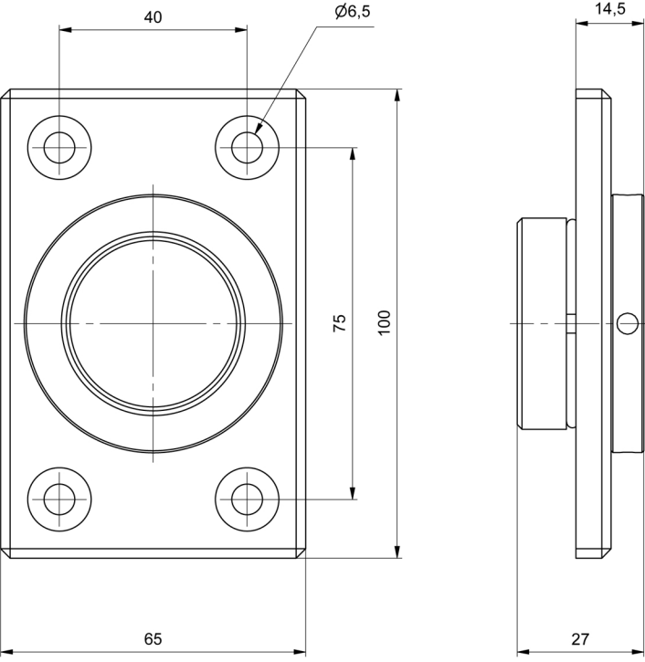
7512 - Bracket Type: 6026-02 Center Mount
