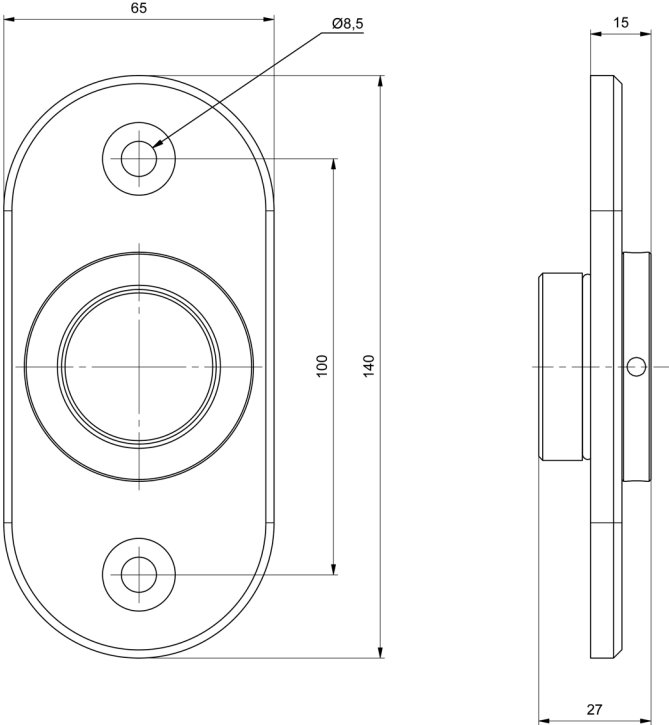
7511 - Bracket Type: 6026-01 Center Mount
