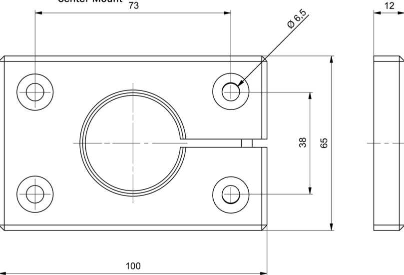
7514 - Bracket Type: 6026-04 Center Mount
