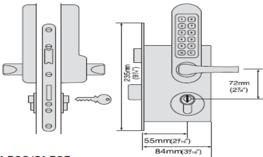
CL520/CL525 with full Panic Function mortice lock and cylinder
